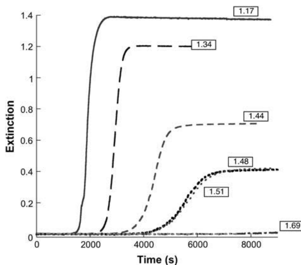
FIGURE 3 Kinetic profiles for insulin gel formation at various pH values (200 \mu\text{M} insulin, 67°C). As the pH decreases, the rate of aggregation and final extinction values increase, whereas the apparent lag time decreases.
