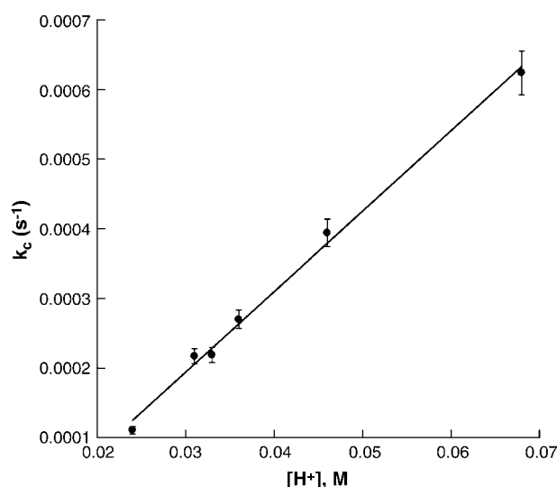
FIGURE 4 Plot of the catalytic rate constant, k_c versus [H^+] for the insulin gelation reactions shown in Fig. 3. The slope of the line is 0.012 \text{ M}^{-1} \text{ s}^{-1} .
