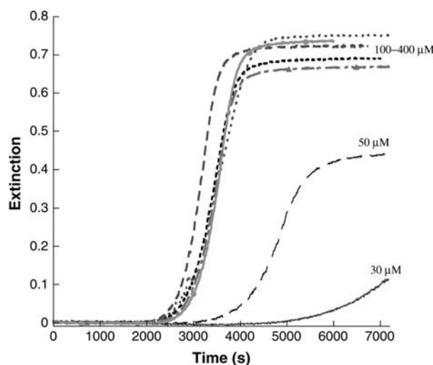
FIGURE 2 Kinetic profiles of gel formation for insulin concentrations between 30 and 400 \mu\text{M} . Equation 3 was adequate to fit these data ( m = 1 ) and n = 10 \pm 1 . For [Insulin] = 30 \mu\text{M} , k_c = 2.0 \times 10^{-4} \text{ s}^{-1} ; [Insulin] = 50 \mu\text{M} , k_c = 2.5 \times 10^{-4} \text{ s}^{-1} and for all higher concentrations, k_c = 3.5 \times 10^{-4} \text{ s}^{-1} .
