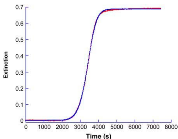
FIGURE 1 Kinetic profile for insulin gelation and the fit provided by Eq. 2. Extinction was measured at 488 nm on a standard spectrophotometer for a solution whose initial conditions were [Insulin] = 200 \mu\text{M} , pH 1.37 at 67°C. The best fit was obtained for k_o \sim 0 ; k_c = 3.8 \times 10^{-4} \text{ s}^{-1} ; n = 11 and m = 1.4 .
