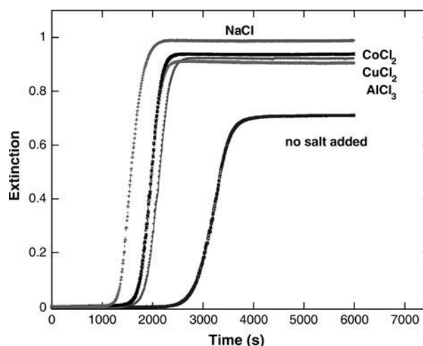
FIGURE 6 Effect of added electrolytes on kinetics of insulin gelation. Each of the salts (NaCl, CuCl_2 , CoCl_2 , and AlCl_3 ) is added so as to make the final ionic strength 0.060 M. The kinetics of gelation is always faster than for a solution to which no electrolyte was added but the difference among electrolytes is minor.
