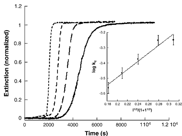
FIGURE 5 Overlay of normalized representative kinetic profiles for insulin gelation at various ionic strengths (NaCl). Shown in the figure (from right to left) are [NaCl] = 0.050, 0.070, 0.10 , and 0.15 . The conditions were 200 \mu\text{M} insulin, pH 1.62, 67^\circ\text{C} . (Inset) Plot of \log k_c versus I^{1/2}/(1 + I^{1/2}) for insulin gelation in the presence of NaCl. The slope of the line is +2.6 \pm 0.3 , indicating interaction between two species of like charge type.
